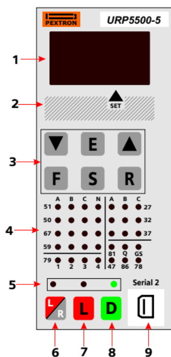
Figura 3.1: Painel frontal.
