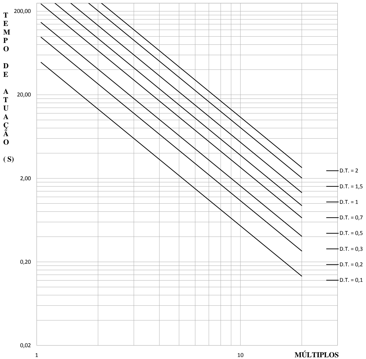
CURVA I2T K = 540 α = 2 β = 0
